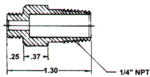
N-76 1/4" NPT P/T Plug
