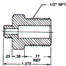
N-78 1/2" NPT P/T Plug
