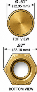
1/8" NPT Test Plug
