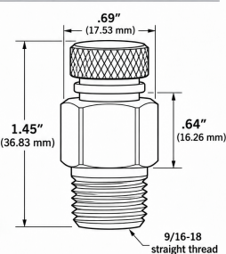
Oil Plug - O-ring seal
